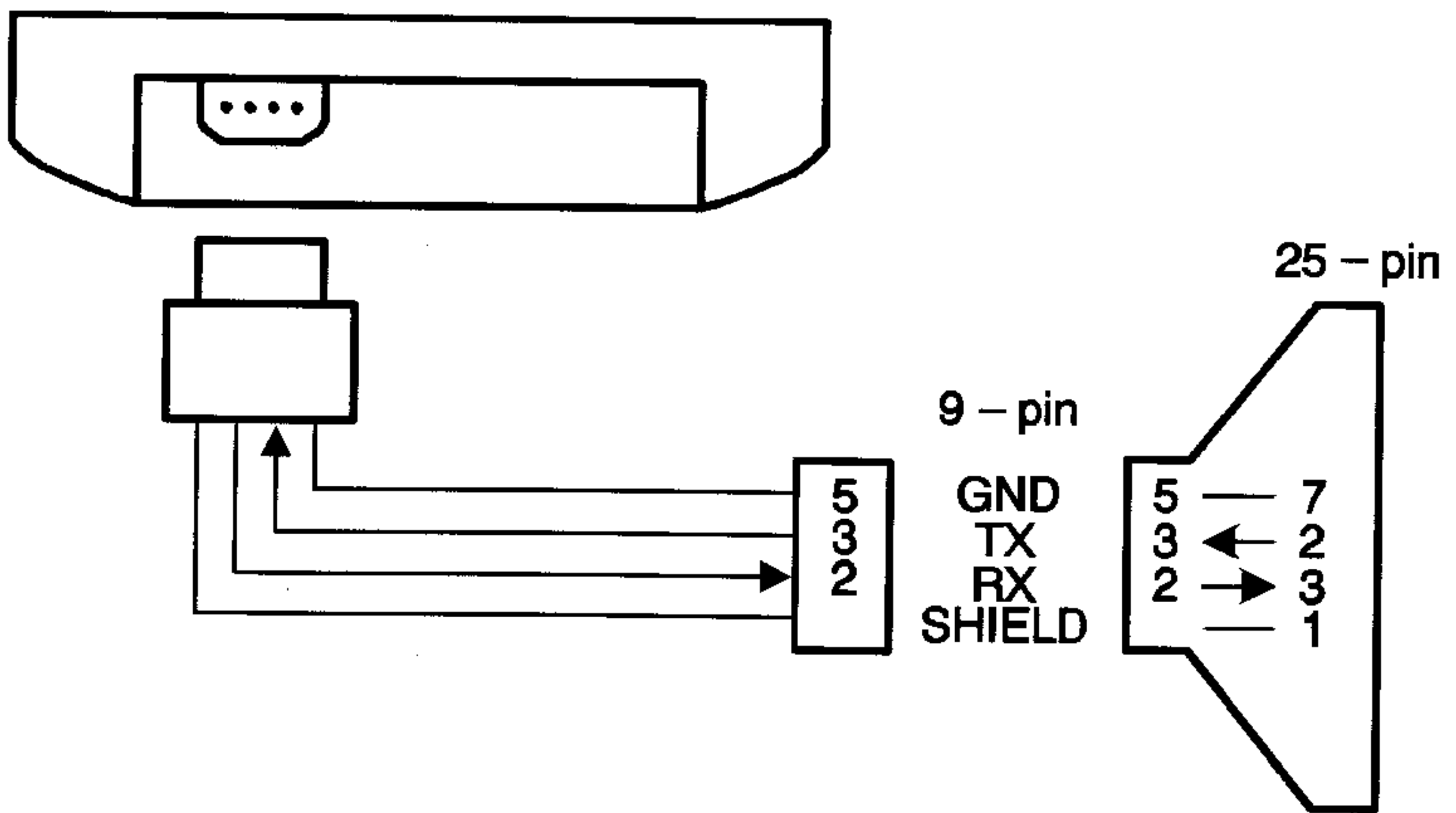
Serial Interface Cable and Adapter (PC Version)
