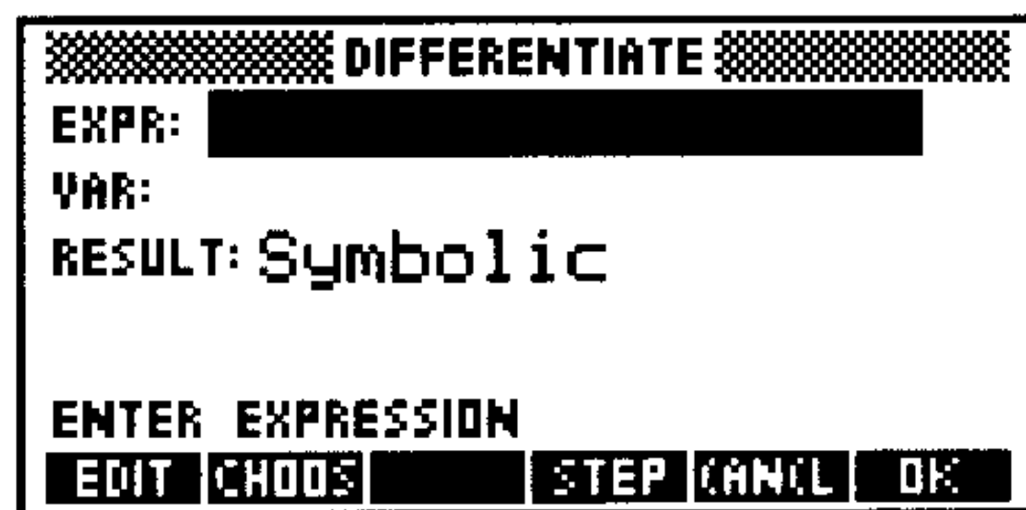
The Symbolic DIFFERENTIATE Screen
